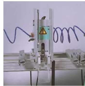
3200P Manual setting of stations and double stacking magazine
