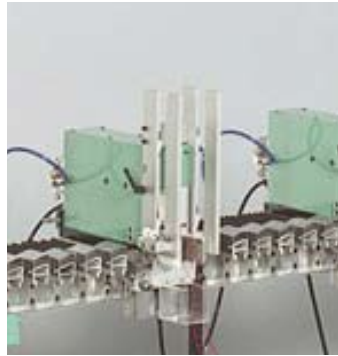
3500P Automatic setting of stations and double stacking magazine
