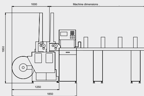
Punching and threading in one station
